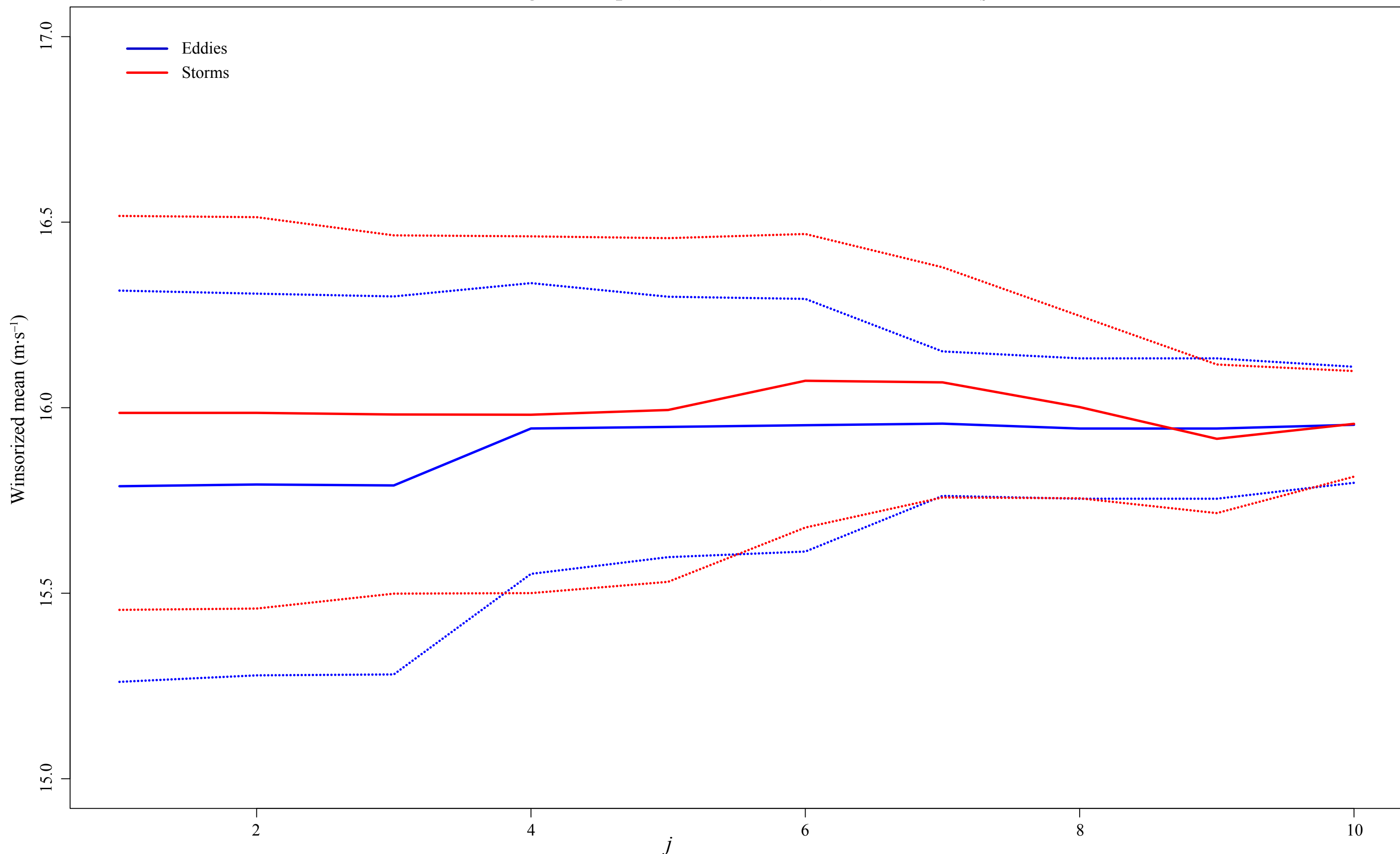
Robustness of central tendency: TES FFISM eddy phase speed (3.7 hPa, 55° S) and MOC-observed dust storm migration speed ( \sim 53^\circ S, mean), MY 24–26, L_s=165\text{--}192^\circ
