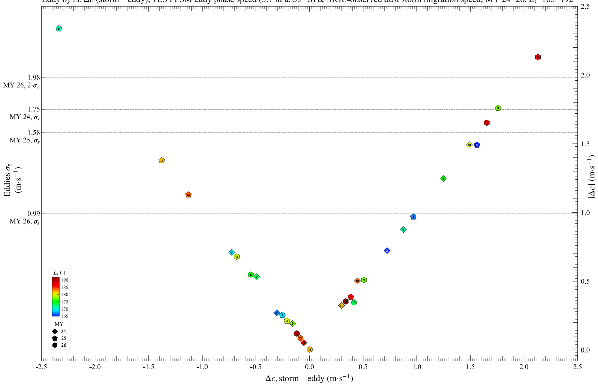
Eddy \sigma_{\bar{x}} vs. \Delta c (storm – eddy), TES FFSM eddy phase speed (3.7 hPa, 55° S) & MOC-observed dust storm migration speed, MY 24–26, L_S=165\text{--}192^\circ
