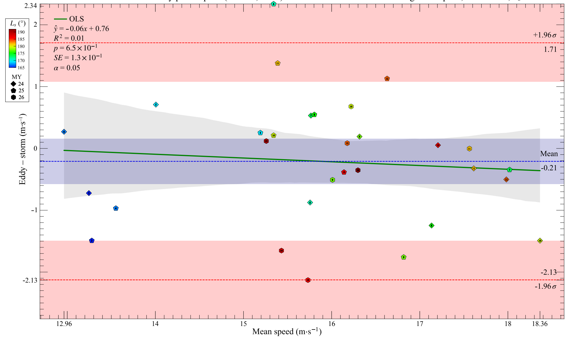
Mean-difference: TES FFSM eddy phase speed (3.7 hPa, 55° S) & MOC-observed dust storm migration speed, MY 24–26, L_s=165\text{--}192^\circ
