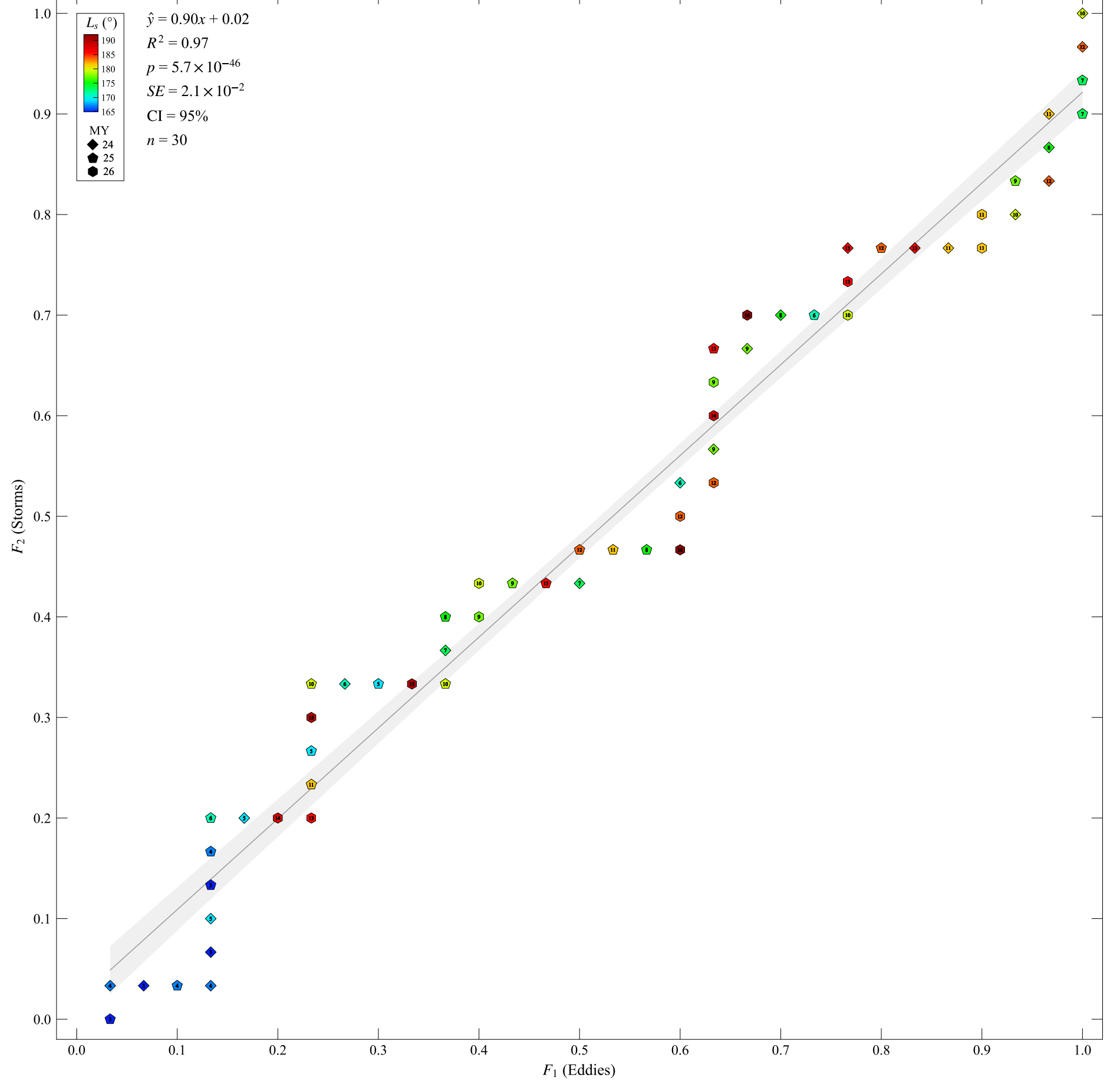
Kolmogorov-Smirnov empirical distribution function, FFSM eddy phase speed (3.7 hPa, 55° S) & MOC dust storm migration speed, MY 24–26, L_s=165-192^\circ
