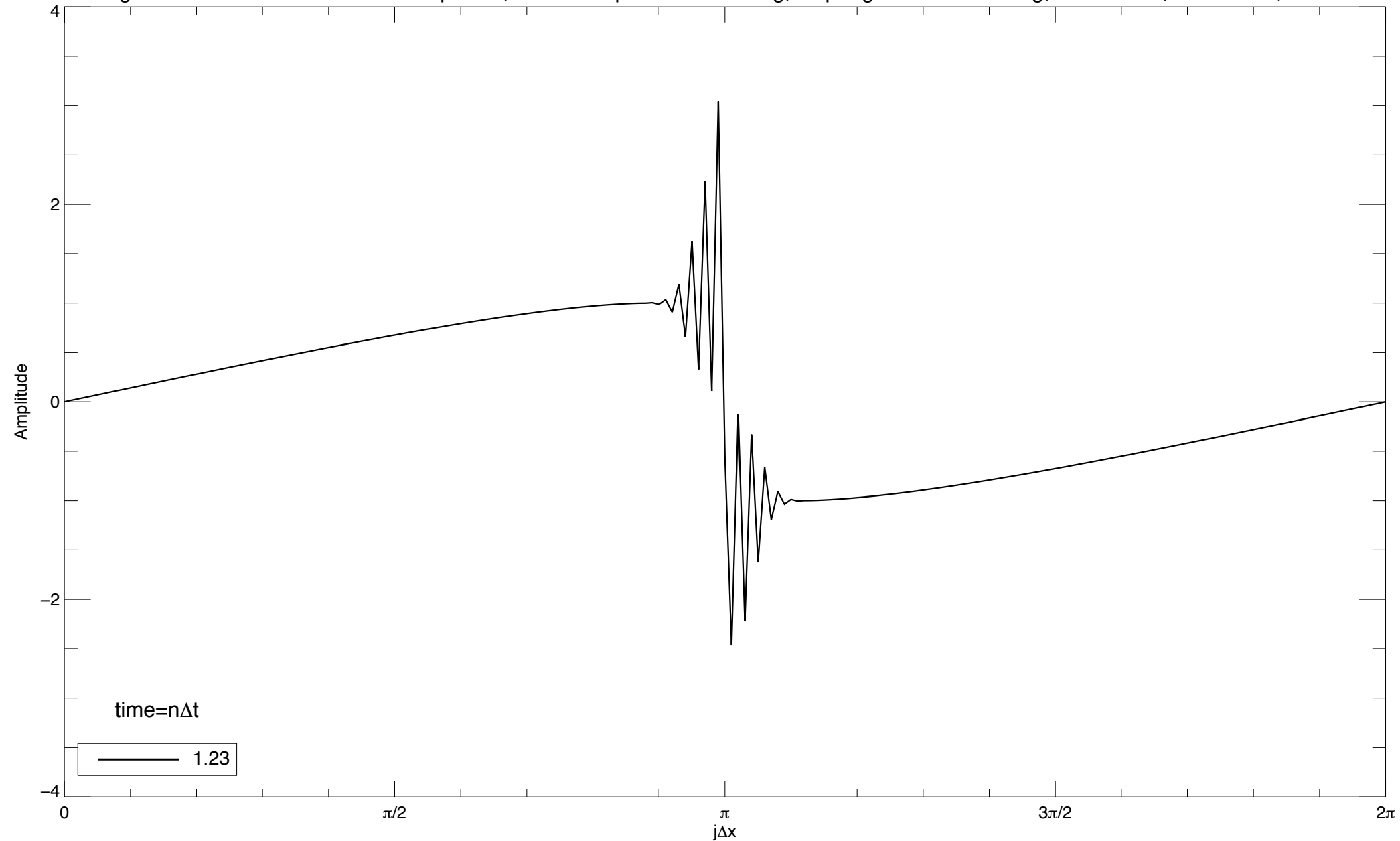
Fig. 4. Non-linear 1-D advection equation, centered space-differencing, leapfrog time-differencing; dx= 0.0314 , dt= 0.0094 , n=130
