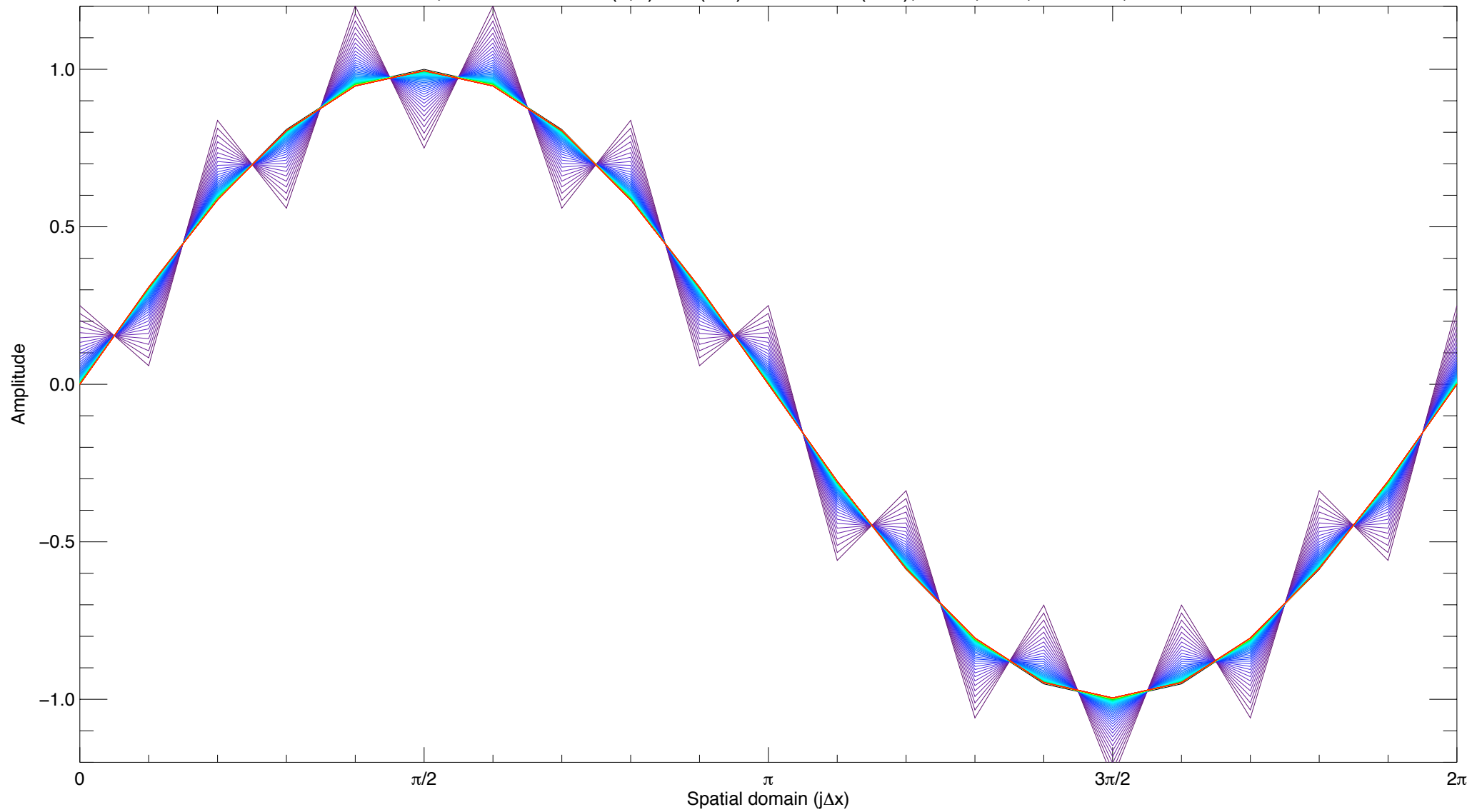
Diffusive filter, 4th order IVP: u(x,0)=\sin(mx) + 0.25*\cos(10x) , n=80,m=1 , \Delta x=\pi/10 , dt= 0.1000
