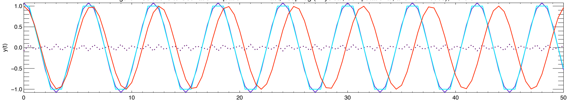
Figure 1 Solutions to Oscillation Equation IVP: Exact, Leapfrog (Physical, Computational, and Full Modes); \Delta t=0.5
