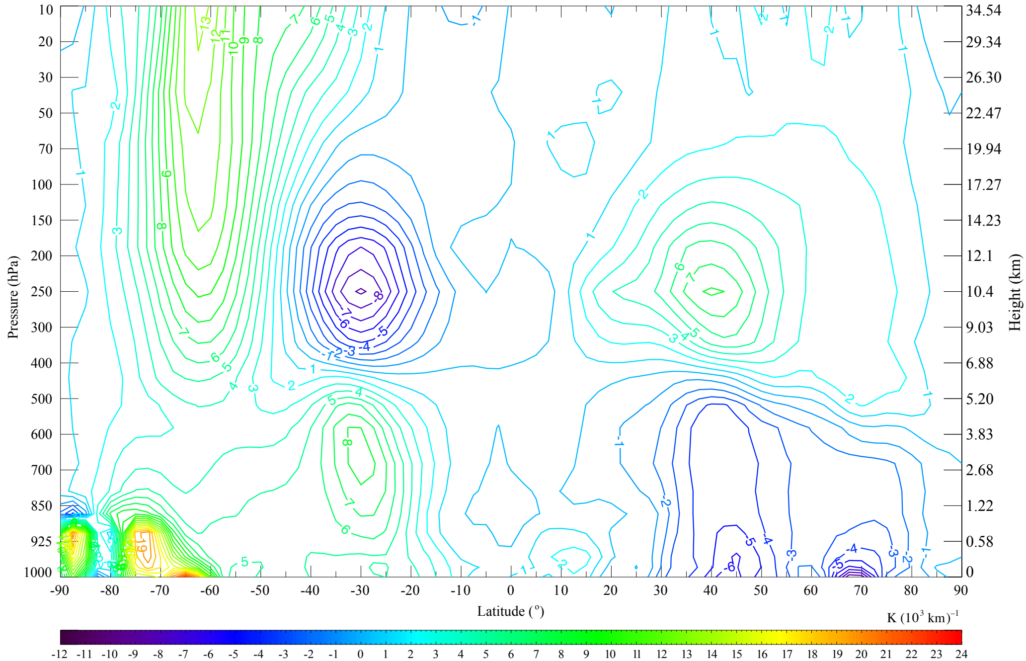
NCEP Reanalysis Meridional Temperature Gradient dT/dy [ \text{K} (10^3 \text{ km})^{-1} ] Cross Section, Jun–Aug 1948–2004
