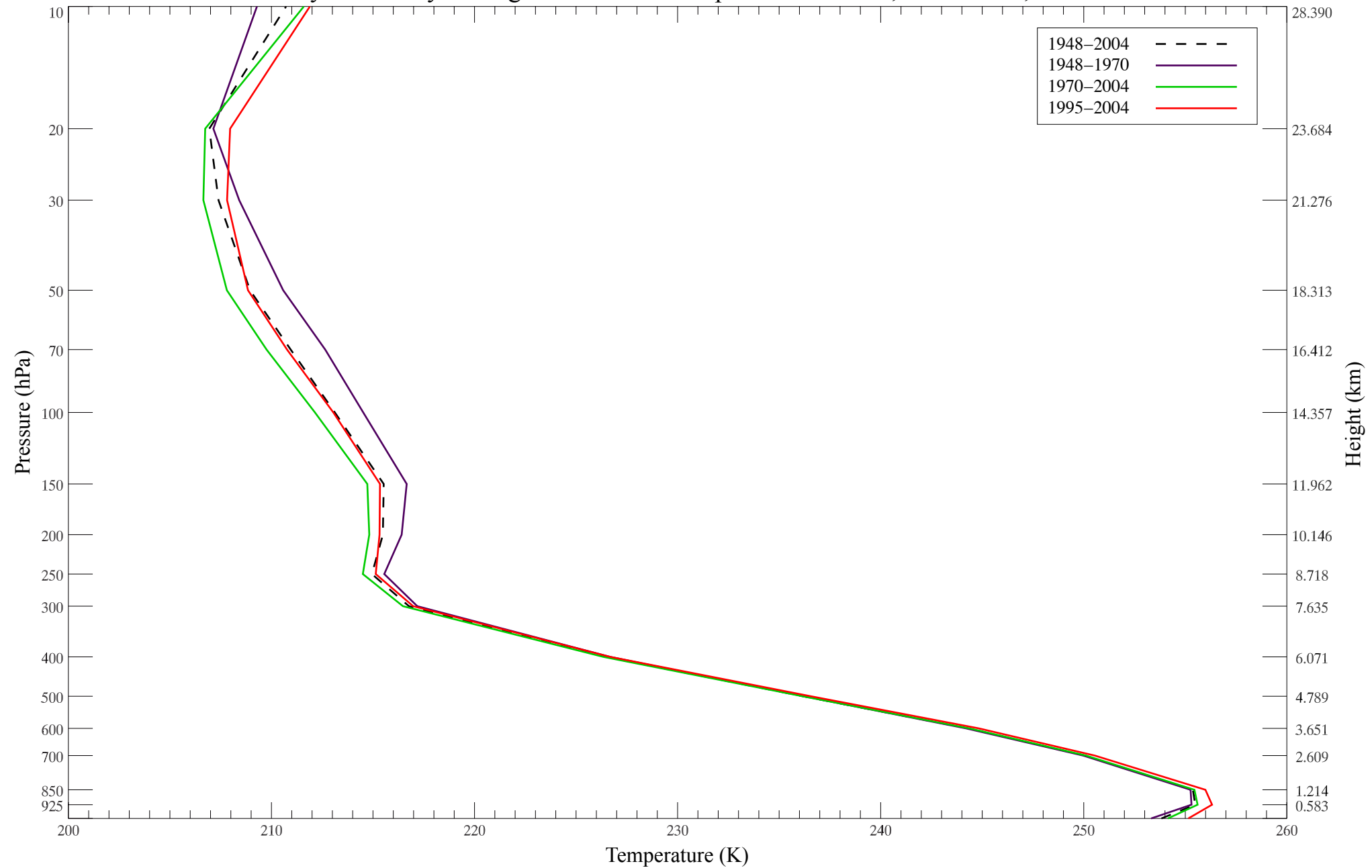
NCEP Reanalysis Zonally Averaged December Temperature Profiles, 1948–2004, Latitude 70° N
