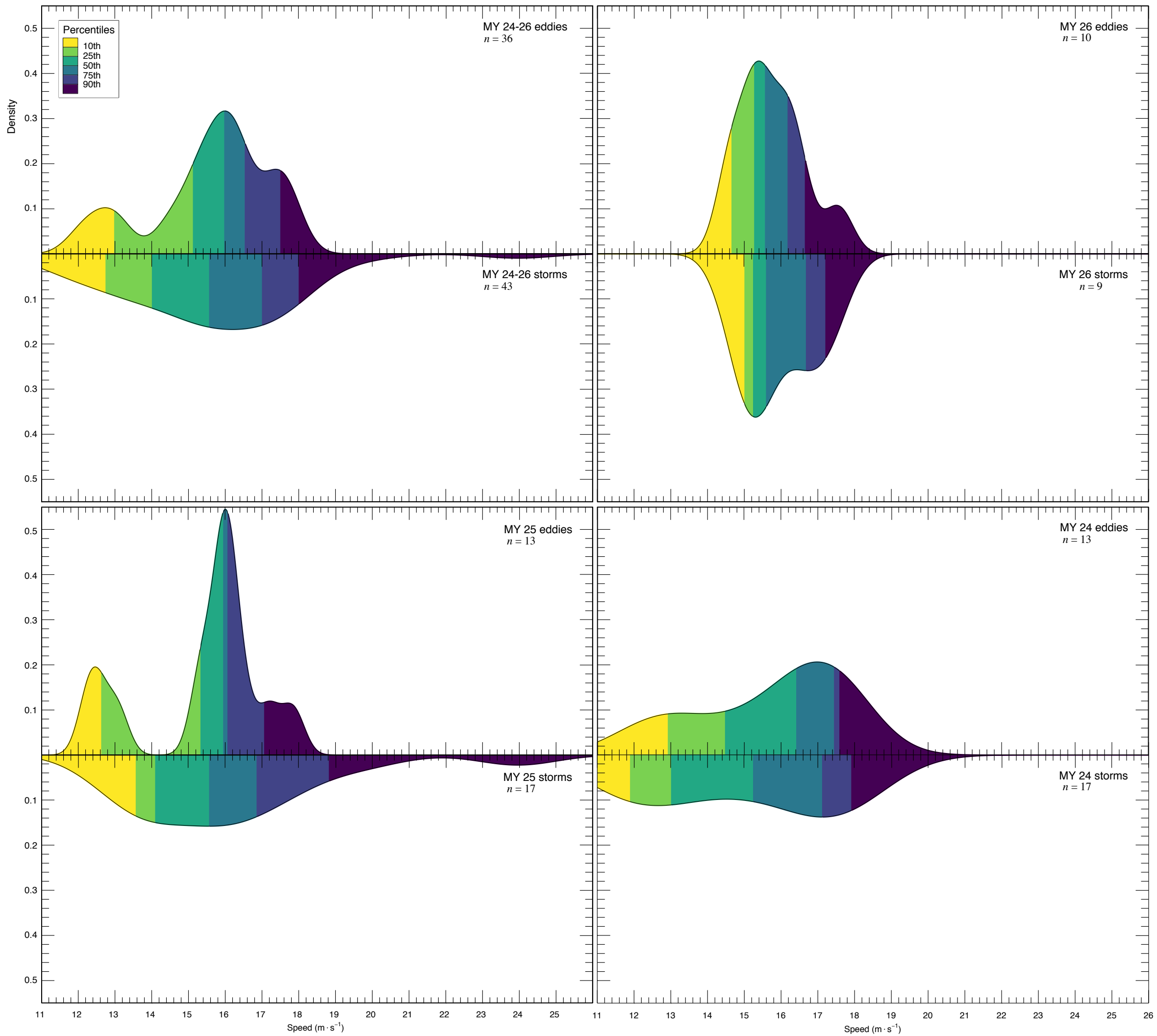
Kernel density estimates of TES FFSM eddy phase speed (3.7 hPa, 55° S) and MOC-observed dust storm migration speed (subset = \Delta \lambda > 180^\circ ), MY 24–26, L_s = 165\text{--}192^\circ
