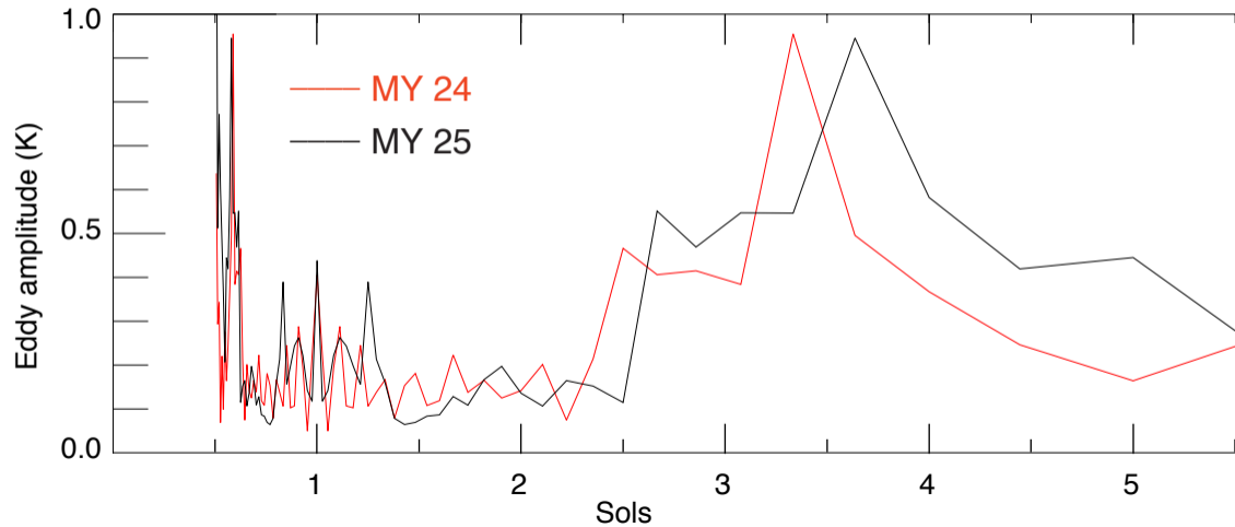
FFT power spectra of TES FFSM eddies in Hellas (40–100° E, 60° S), MY 24 & 25
