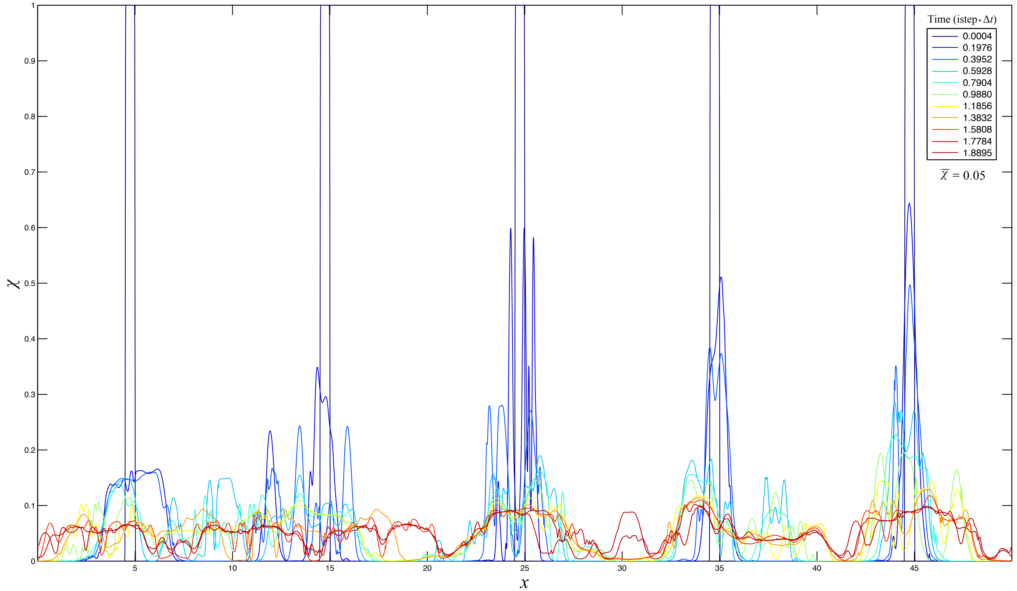
Time evolution of \chi (mixing fraction of clear air)
