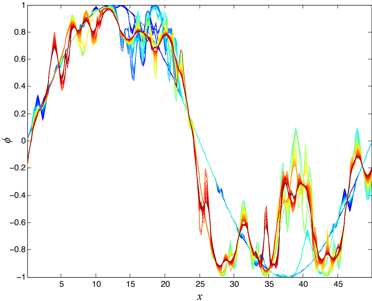
\sin(x) time evolution, t = 20
