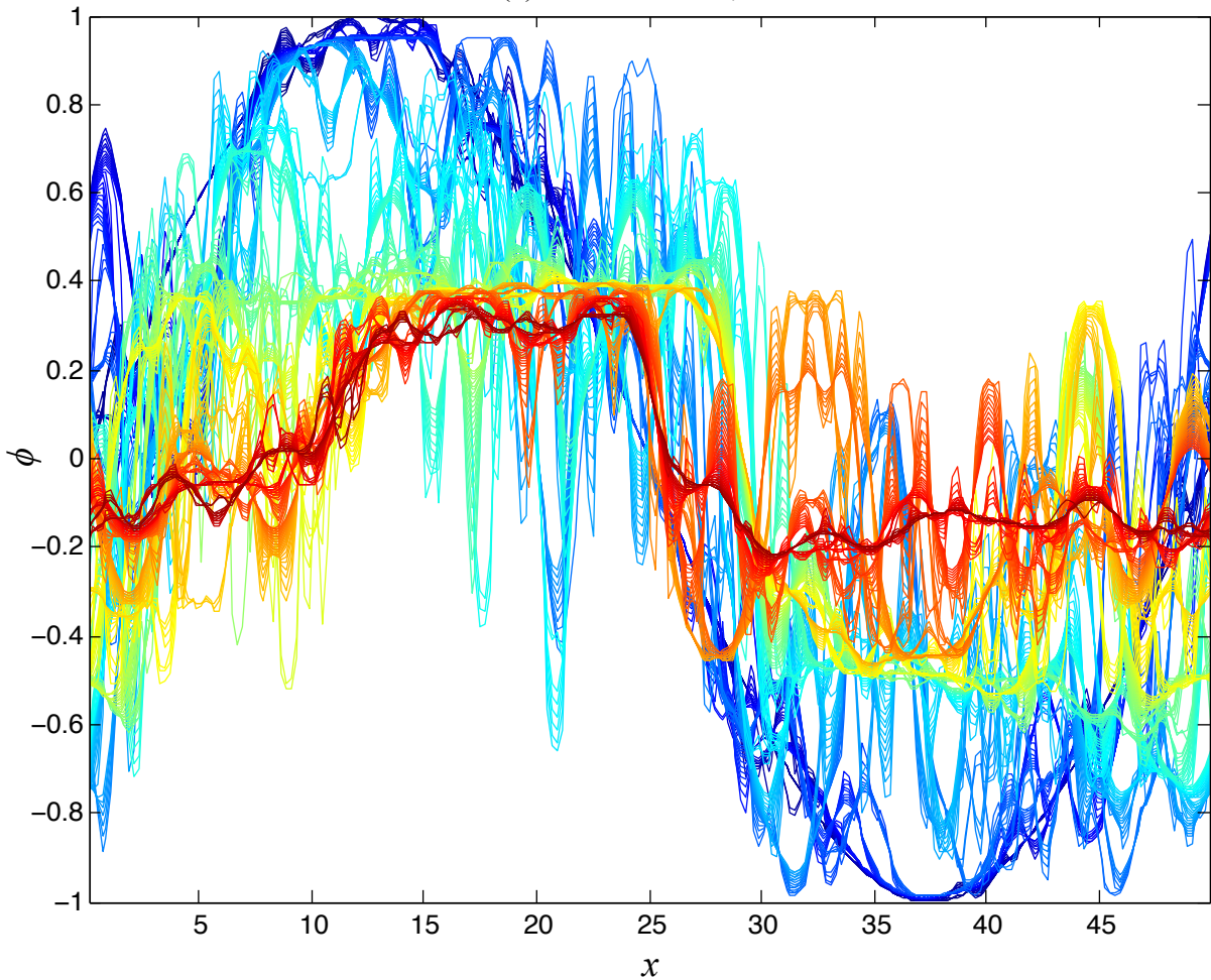
\sin(x) time evolution, t = 140
